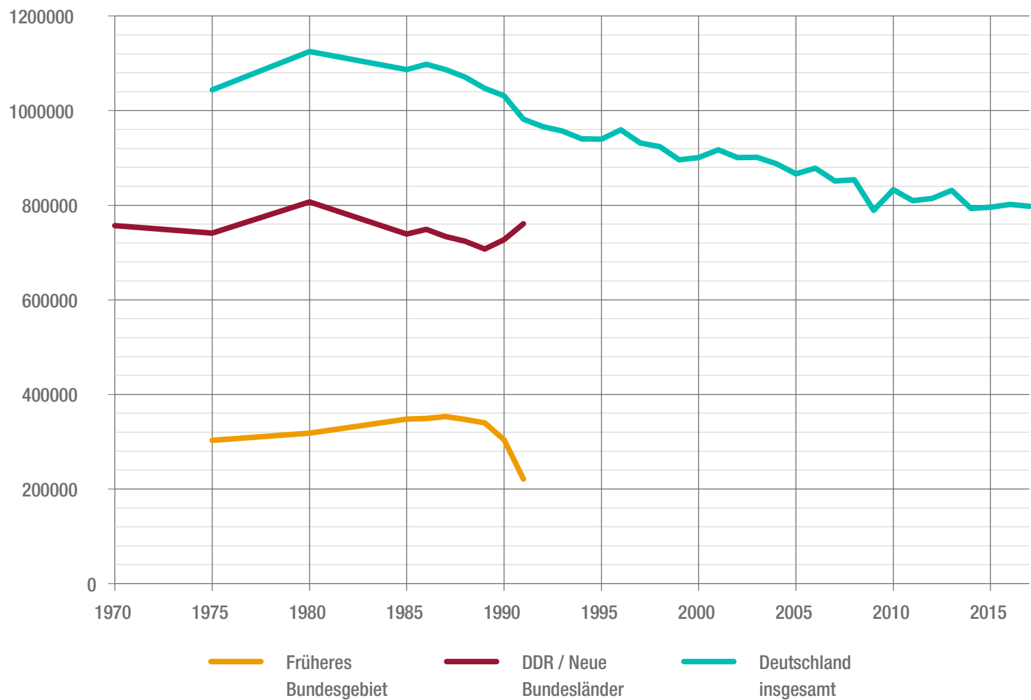
Kohlendioxid-Emissionen in Kilotonnen (CO2 in kt) 1970-2017
